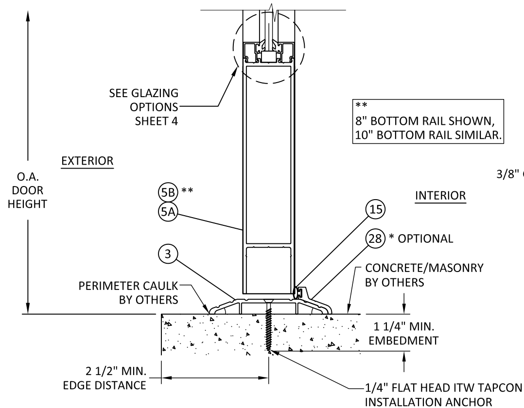
A 4 VERTICAL SECTION BOTTOM RAIL - CONCRETE/MASONRY
