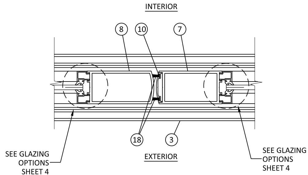
F 5 HORIZONTAL SECTION MEETING STILE
