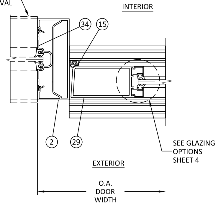
L 5 HORIZONTAL SECTION JAMB - STOREFRONT INSTALLATION
