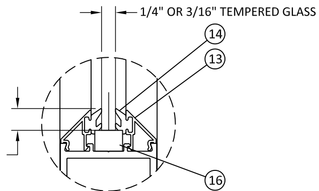
GLAZING DETAIL B
