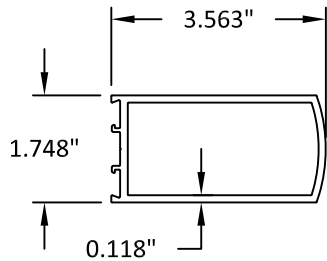
8 MEETING STILE (INACTIVE)
