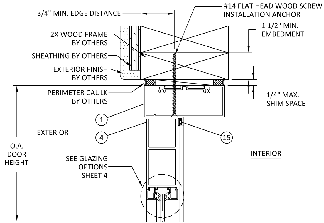
B 4 VERTICAL SECTION DOOR HEAD - 2X WOOD FRAME
