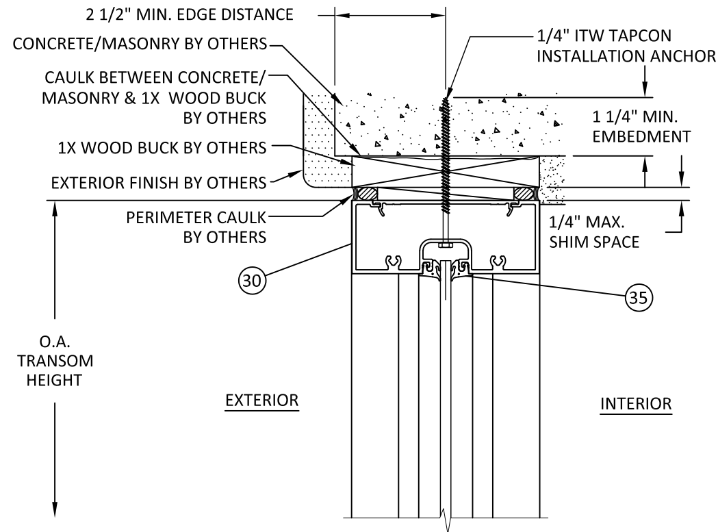
H 6 VERTICAL SECTION HEAD - CONCRETE/MASONRY
