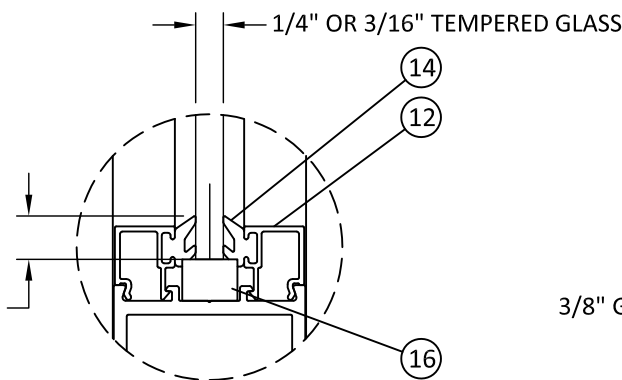
GLAZING DETAIL A
